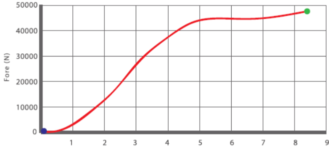
COMPRESSION TEST (HOT 23°)
