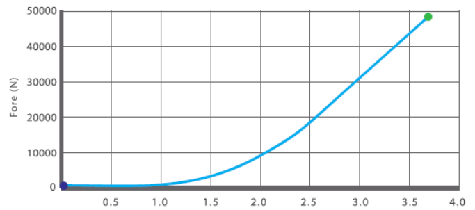
COMPRESSION TEST (COLD -40°)
