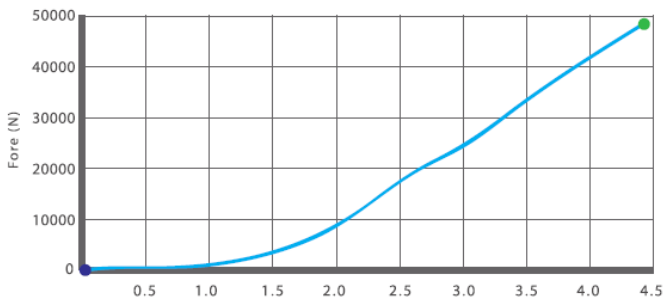
COMPRESSION TEST (COLD -40°)
